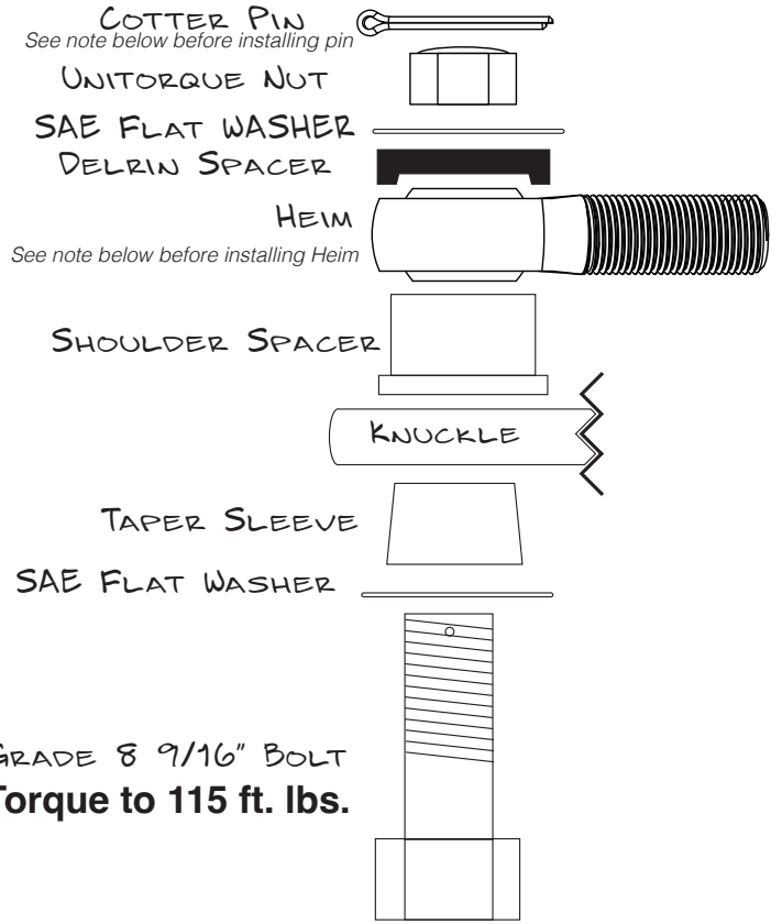
Tie Rod Over (TRO)
