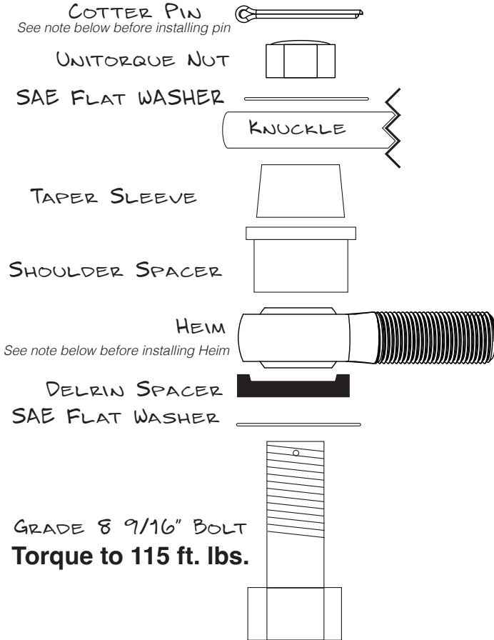
Tie Rod Under (TRU)
